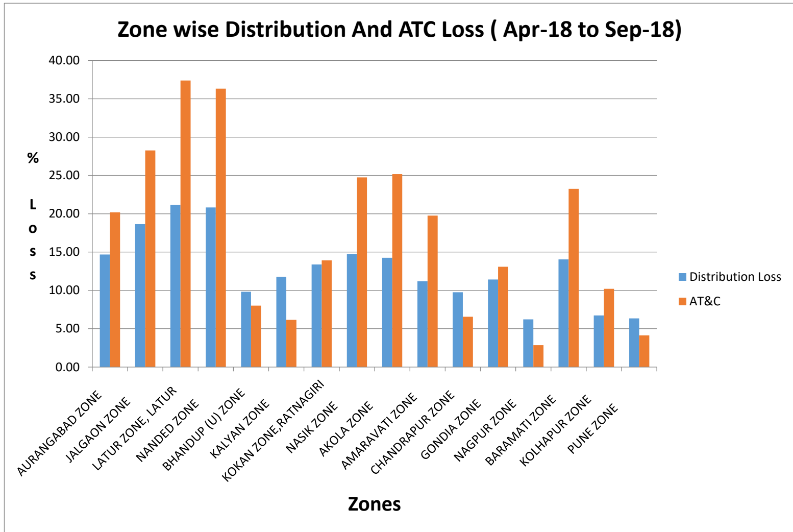
Zone wise Distribution Loss and ATC for the period Apr-18 to Sept-18 ( Provisional)
